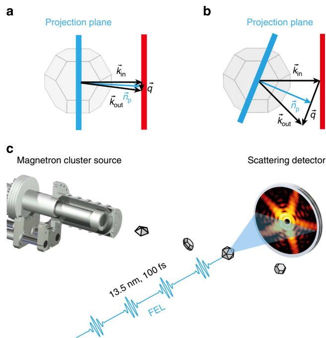
Figure 1 | Schematics of the wide-angle scattering experiment. In Born's approximation, the far-field scattering intensity reads I(\mathbf{q}) \propto |\int \rho(\mathbf{r}) e^{i\mathbf{q} \cdot \mathbf{r}} d^3r|^2 , where \rho(\mathbf{r}) is the scattering density of the particle centered at \mathbf{r} = 0 . After decomposing \mathbf{r} into components parallel ( \mathbf{r}_{||} ) and perpendicular ( \mathbf{r}_{\perp} ) to the projection vector \mathbf{n}_p = \mathbf{k}_{in} + \mathbf{q}/2 , which is by definition perpendicular to \mathbf{q} , the intensity can be recast as I(\mathbf{q}) \propto |\rho(\mathbf{r}_{\perp}) e^{i\mathbf{q} \cdot \mathbf{r}_{\perp}} d^2r_{\perp}|^2 , representing the Fourier transform of the projected density \rho(\mathbf{r}_{\perp}) = \int \rho(\mathbf{r}) d^3r_{||} on a plane with normal vector \mathbf{n}_p . (a) For small scattering angles, the approximation \mathbf{n}_p \parallel \mathbf{k}_{in} is valid, which inhibits access to any structural information along this direction. (b) The variation of \mathbf{n}_p with \mathbf{q} for large scattering angles provides access to the 3D properties of the particle. (c) In the experiment, single-shot diffraction patterns of silver particles intersecting the FEL photon beam are captured by the 2D detector.
